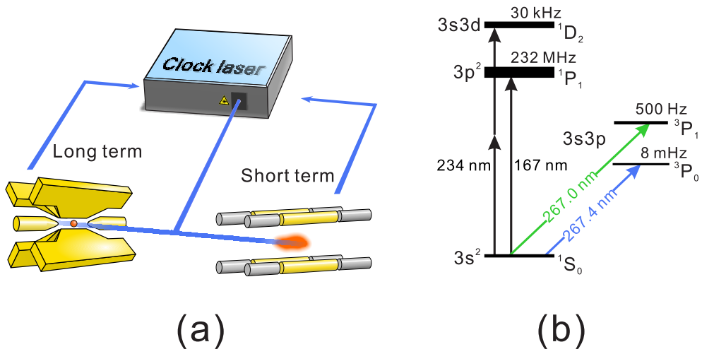
FIG. 1: (Color online) (a) Proposed Al + ions optical clocks scheme. (b) Energy levels and relevant transitions of Al + ions.
