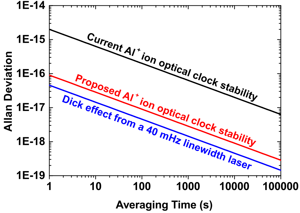
FIG. 2: (Color online) Comparison of clock laser stability. The black line is the current Al + ion optical clock performance level of 2.0 \times 10^{-15}/\sqrt{\tau} , and the red line is the expected clock laser stability improvement level of 9.0 \times 10^{-17}/\sqrt{\tau} . For comparison, the Dick effect contribution from a 40 mHz line width laser (probe time 0.8 s, dead time 0.2 s) is shown as the blue line.
