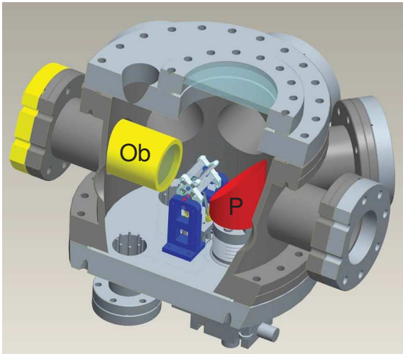
Fig. 5 Schematic cross section of the vacuum setup. Fluorescence from the ion stored in the Paul trap (center) is collected via an UV objective (Ob) and a parabolic mirror (P). The objective is mounted inside an inverted viewport to minimize the distance to the ion for higher collection efficiency. Both channels are imaged outside the vacuum chamber onto a single PMT, yielding their combined count rates.
